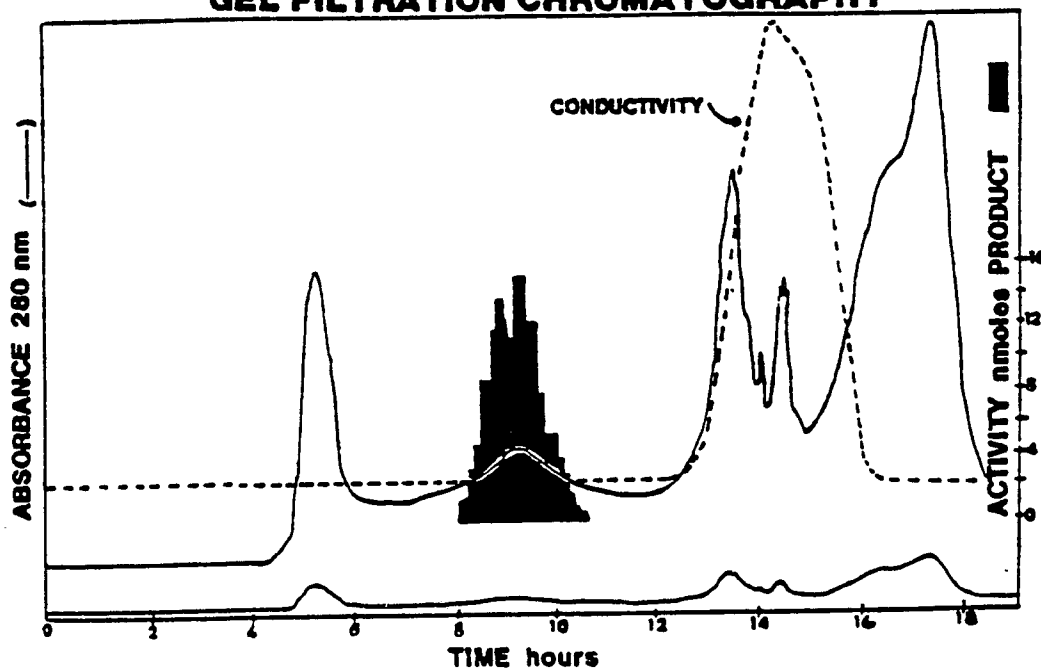
GEL FILTRATION CHROMATOGRAPHY
