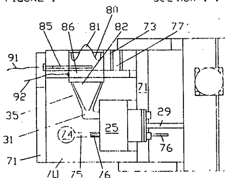
FIGURE 1 Section 1-1'
