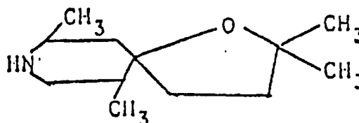
2,2,6,9-tetramethyl-1-oxa-8-azaspiro[4.5]decane
