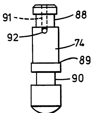
FIG. 8 PRIOR ART
