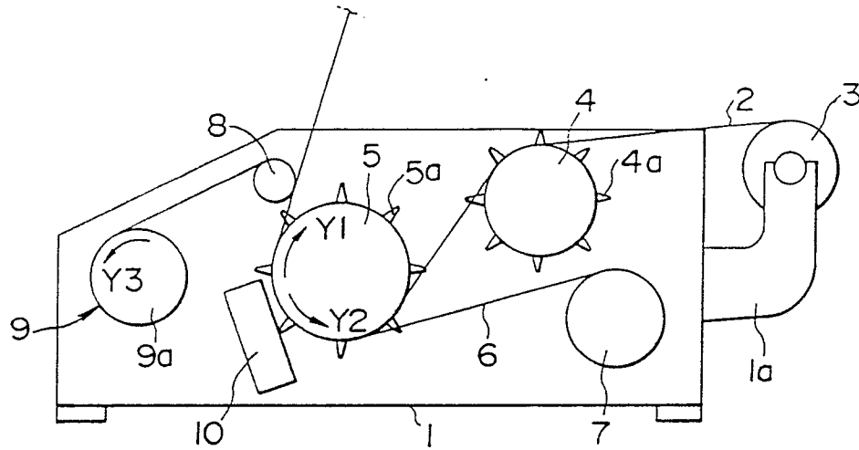
FIG.2 (PRIOR ART)
