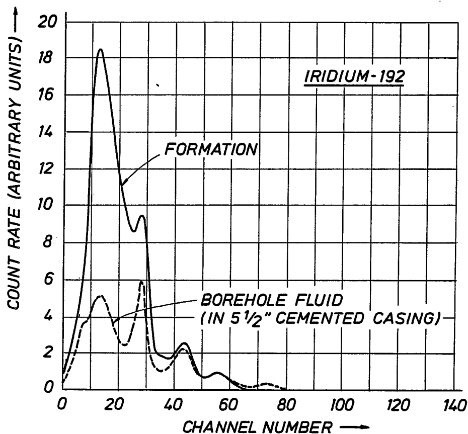
FIG.2 FORMATION AND BOREHOLE SPECTRA FOR ^{192}\text{Ir}
