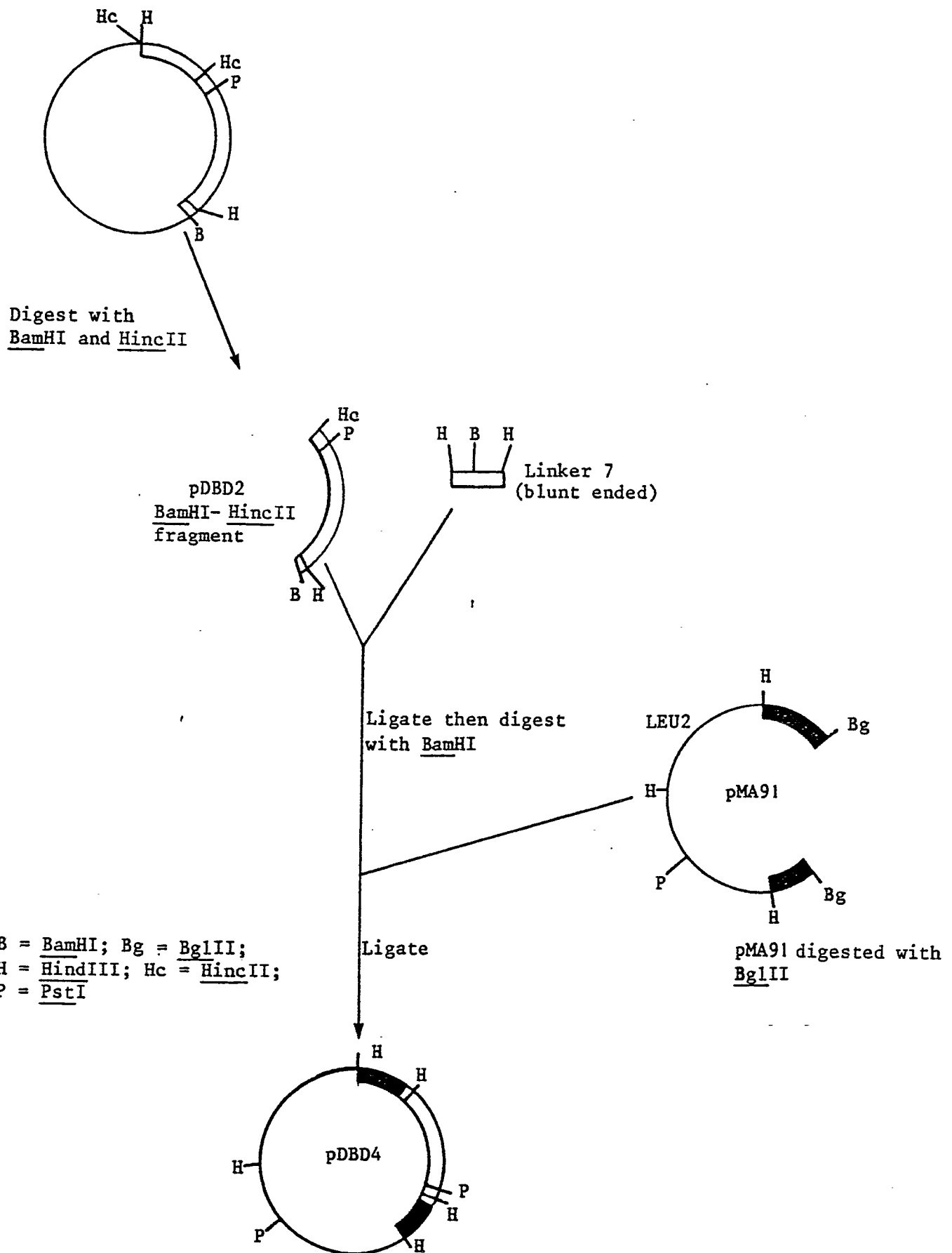
FIGURE 7 Construction of pDBD4
