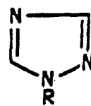
1, 2, 4-Triazole
