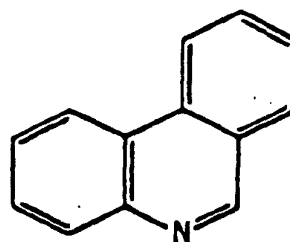
Phenanthridine
