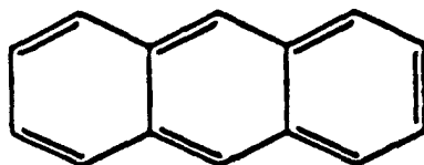
Anthracenes
