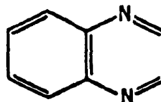
Quinoxaline
