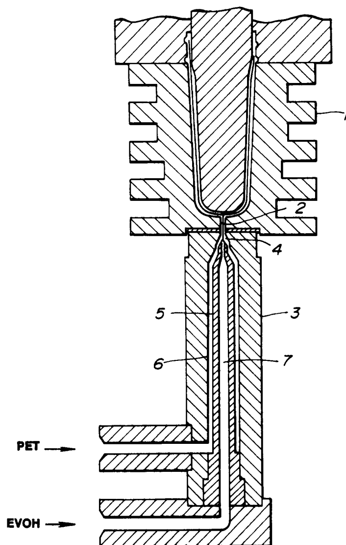
FIG. 7 (PRIOR ART)
