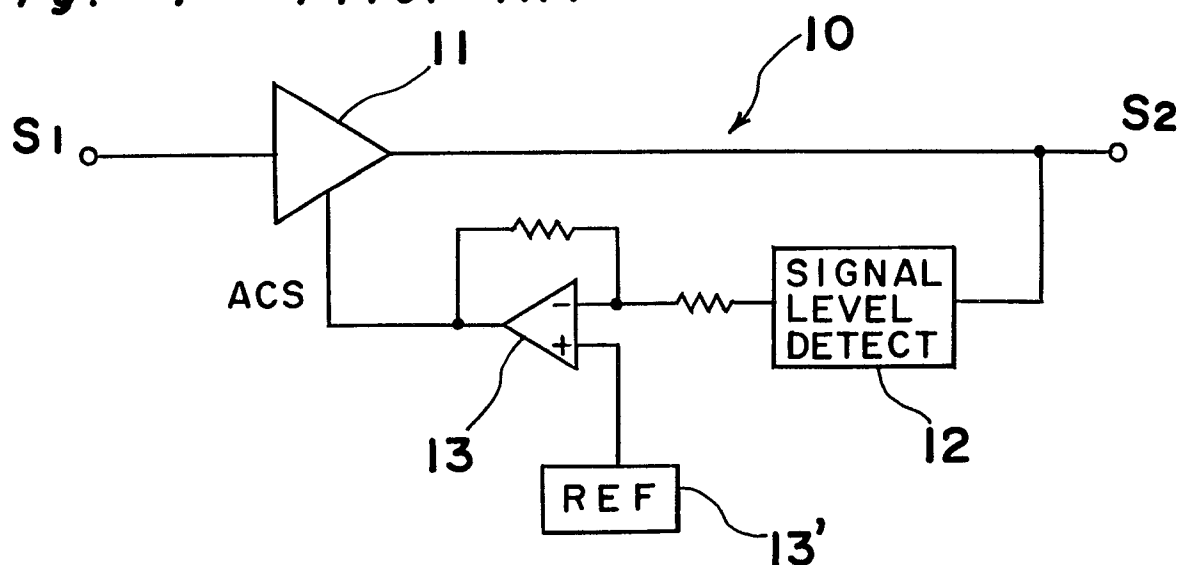
Fig. 4 Prior Art
