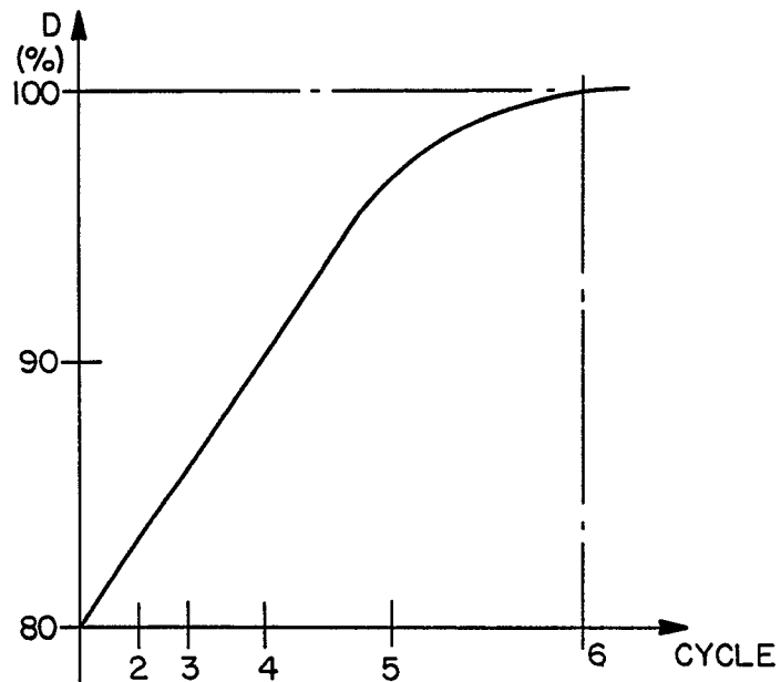
FIG.2D DRYNESS LEVEL/CYCLE
