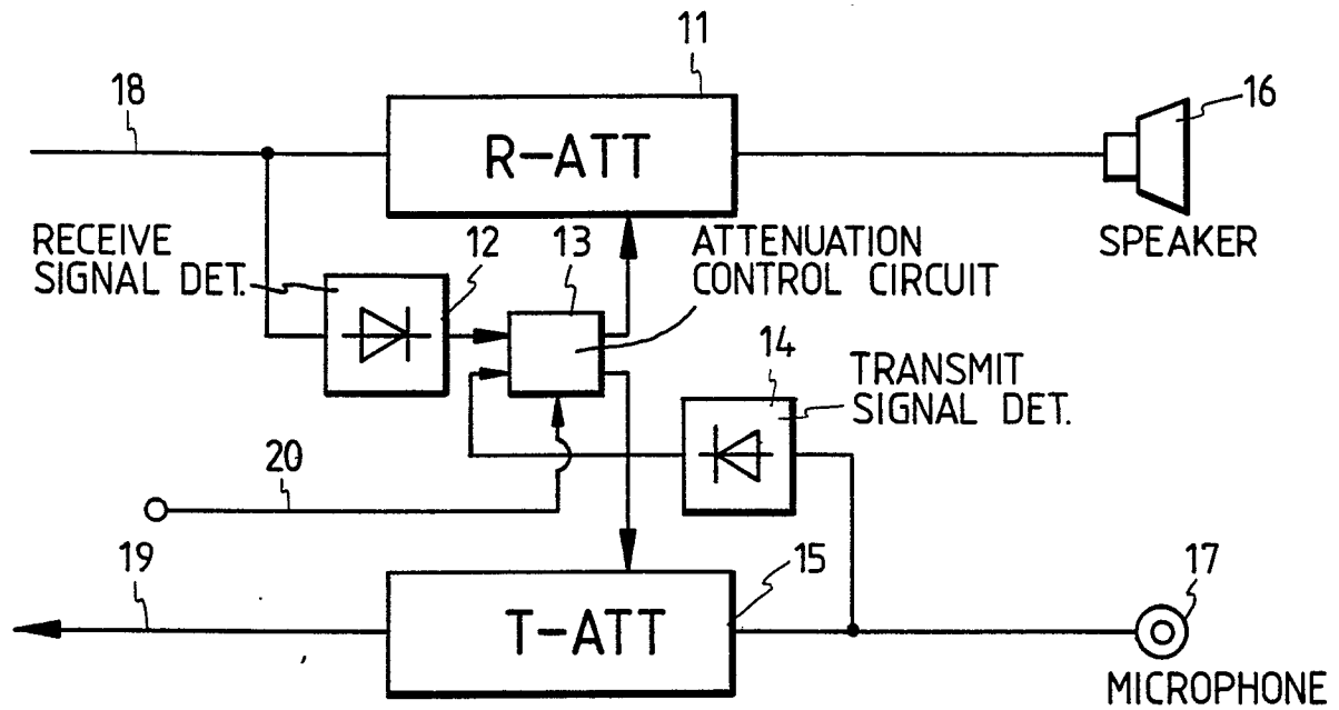
FIG. 1. PRIOR ART
