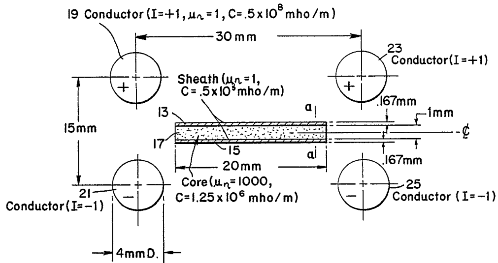
IDEALIZED MODEL OF NEEDLE & INDUCTION COILS
