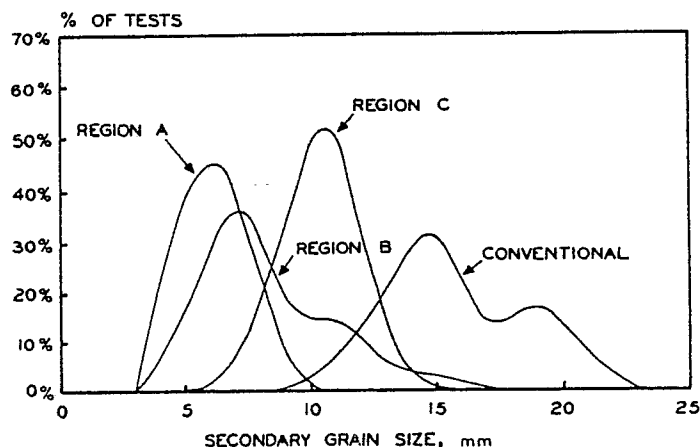
FIG. 2 GRAIN SIZE DISTRIBUTION VERSUS ULTRA-RAPID HEATING REGION
