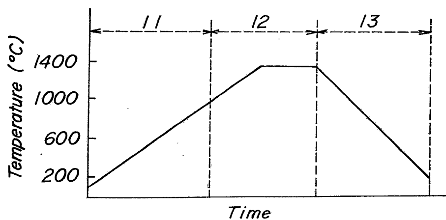
FIG. 5 PRIOR ART
