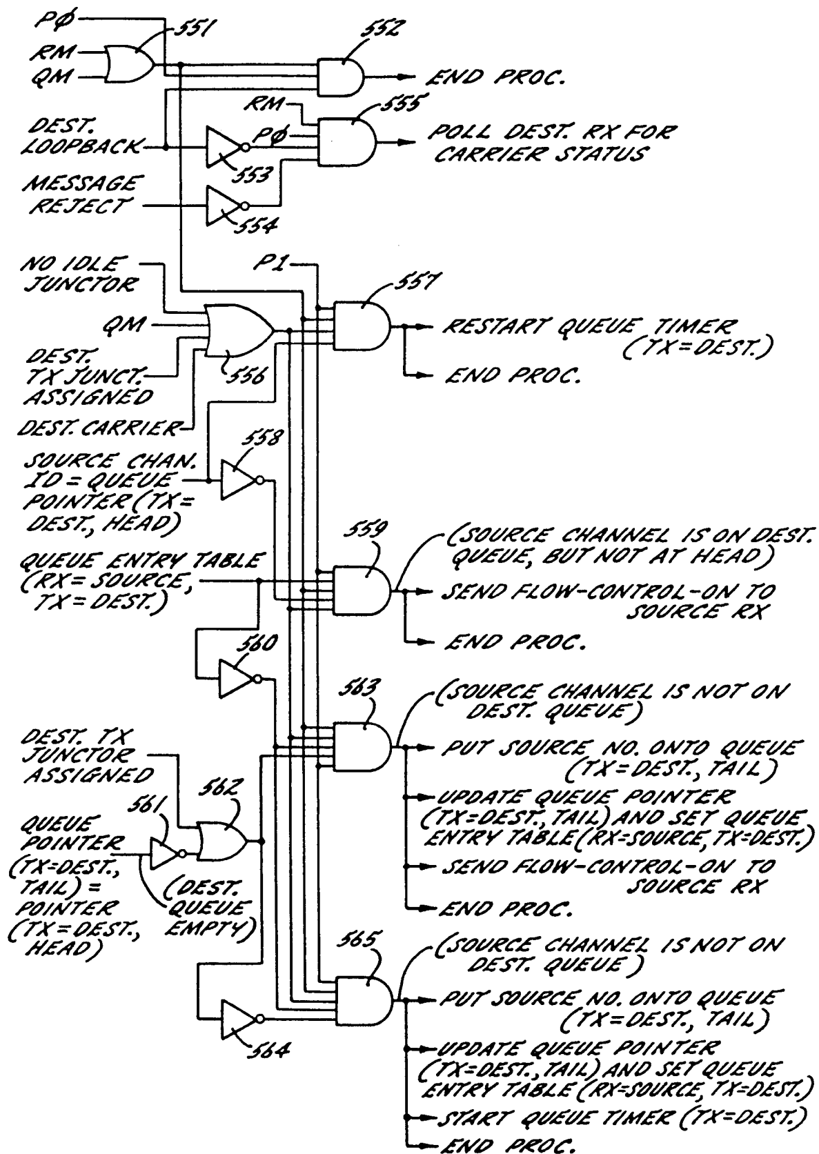
COMBINATIONAL LOGIC FOR MESSAGE QUEUING
