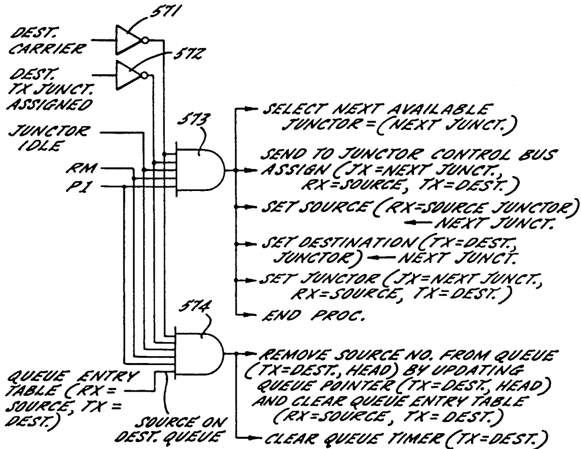
COMBINATIONAL LOGIC FOR ROUTING MESSAGE
