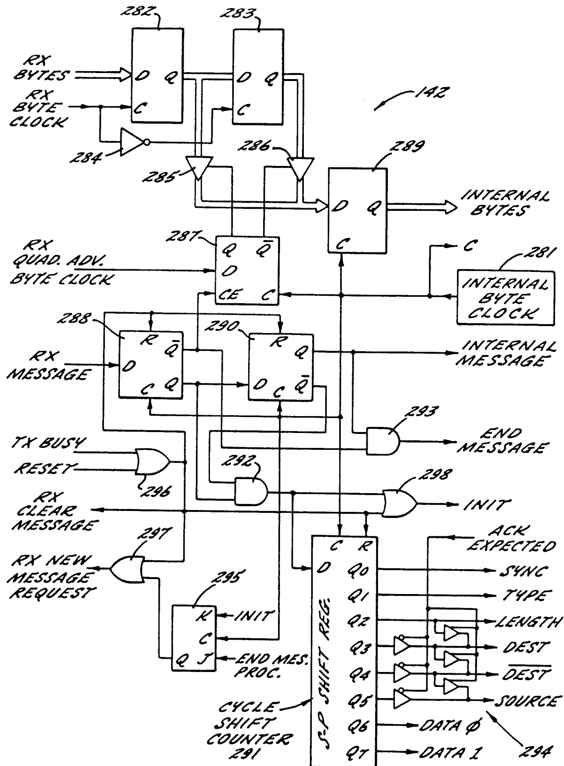
RX LOGIC MESSAGE SYNCHRONIZER AND CYCLE COUNTER
