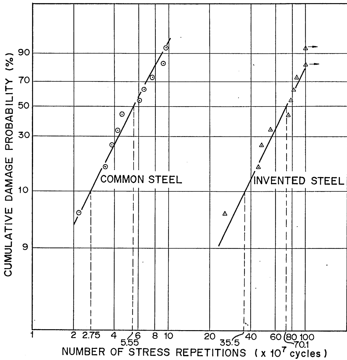
WEIBULL CHART
