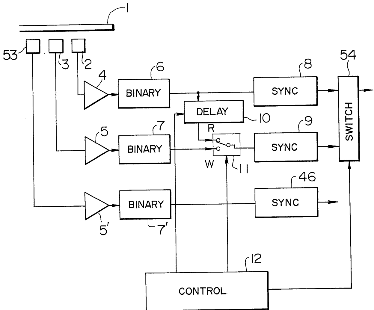
FIG. 3 DELAYING CLOCK SIGNAL
