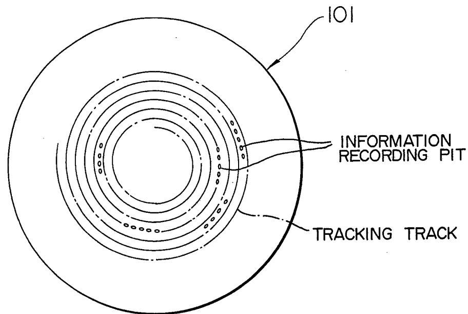
FIG. 7 SPIRAL TRACK DISK
