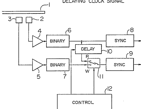
FIG. 1 DELAYING CLOCK SIGNAL
