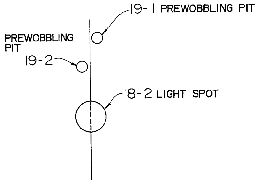
FIG. 10 SAMPLE SERVO SYSTEM
