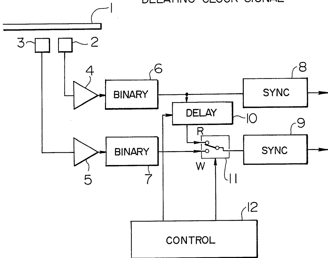
FIG. 1 DELAYING CLOCK SIGNAL
