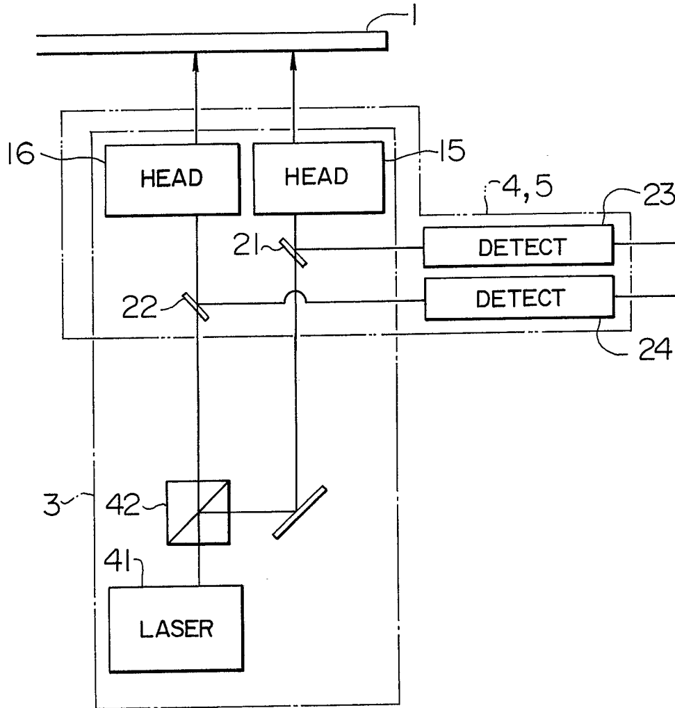
FIG. 5 INTEGRAL FORMATION OF DETECTOR
