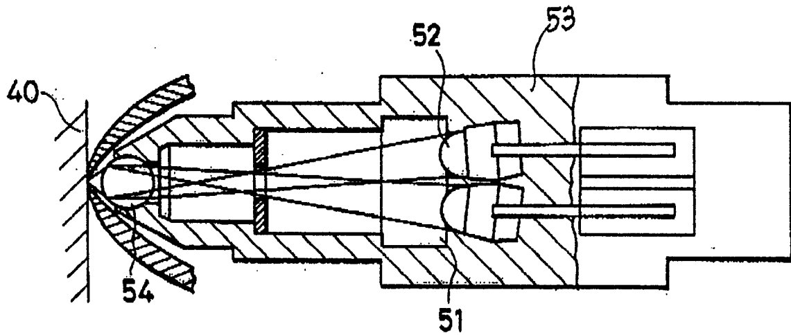
FIG. 6 (Prior Art)
