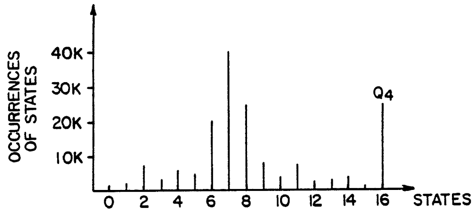
FIG. 9 : HISTOGRAM OF CHARACTERISTIC SIGNALS (CS)
