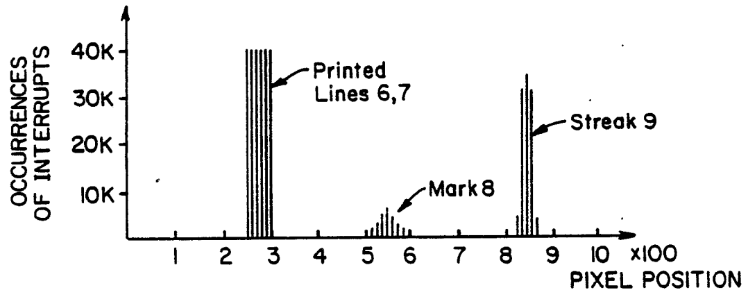
FIG. 10 : HISTOGRAM OF INTERRUPT SIGNALS (I)
