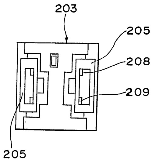
Fig. 24 PRIOR ART
