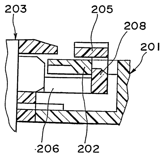
Fig. 25 PRIOR ART
