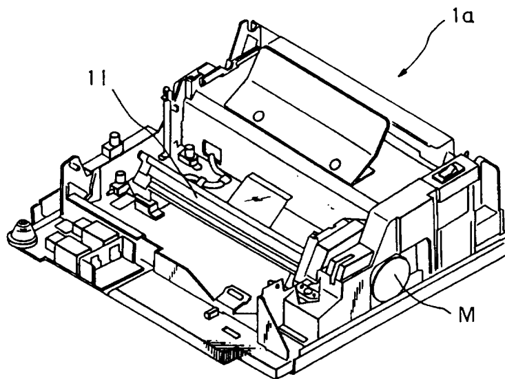
Fig. 12 ( PROCESS CARTRIDGE REMOVED )
