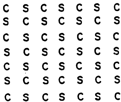
\beta SiC
