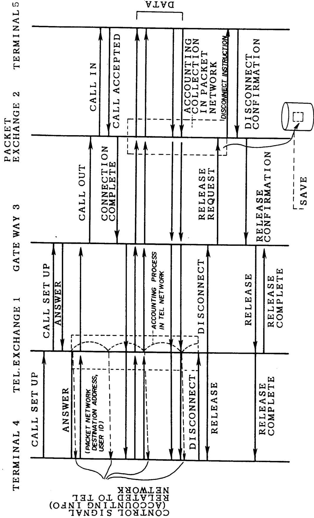
FIG.2 PRIOR ART
