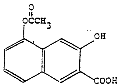
g) 5-acetoxy-3-hydroxy-2-naphthoic acid
