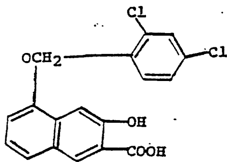
t) 5-(2,6-dichlorobenzyloxy)-3-hydroxy-2-naphthoic acid
