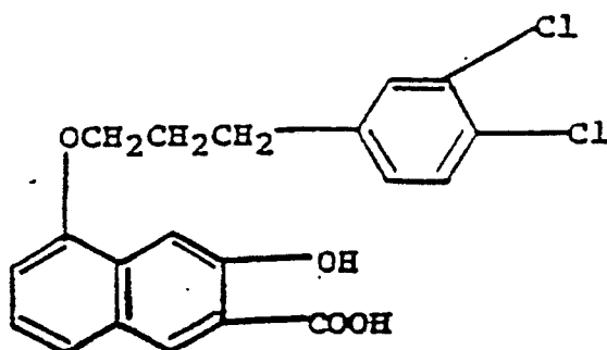
v) 5-(4-fluorobenzyloxy)-3-hydroxy-2-naphthoic acid
