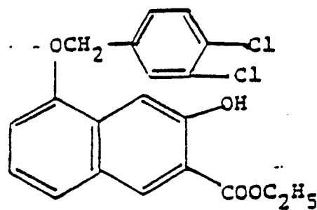
f) ethyl 5-(3,4-dichlorobenzyloxy)-3-hydroxy-2-naphthoate
