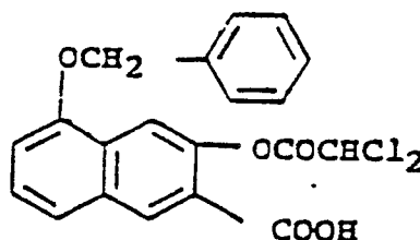
y) 5-benzyloxy-3-dichloroacetoxy-2-naphthoic acid
