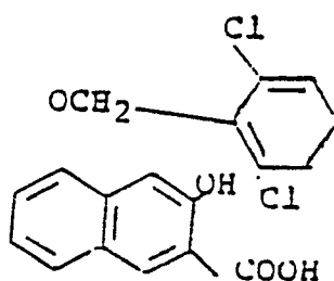
t) 5-(2,6-dichlorobenzyloxy)-3-hydroxy-2-naphthoic acid
