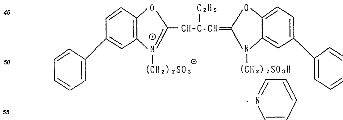
Sensitizing Dye VII
