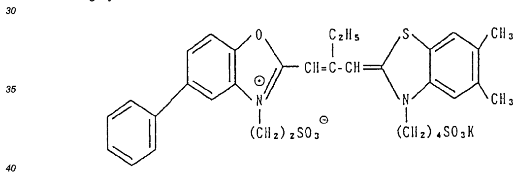
Sensitizing Dye VI
