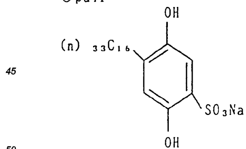
C pd A
