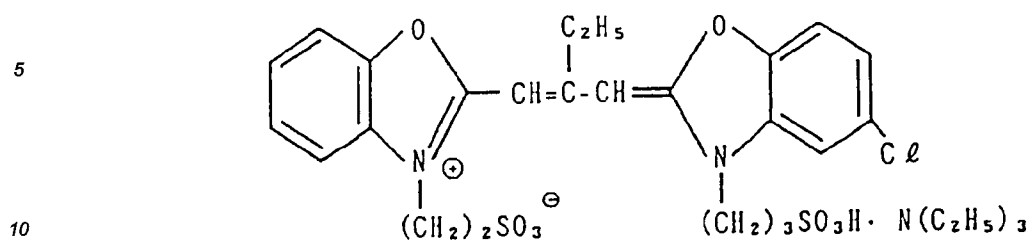
Sensitizing Dye V
