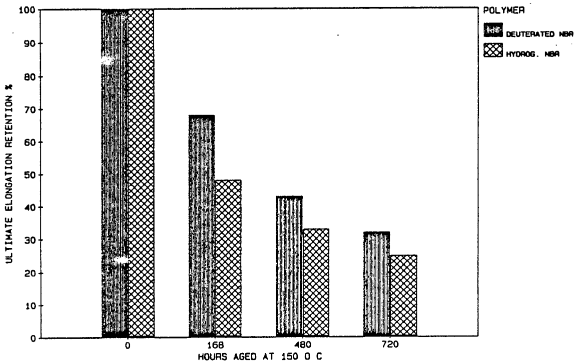
FIGURE 1 AIR AGING OF DEUTERATED AND HYDROGENATED NBR
