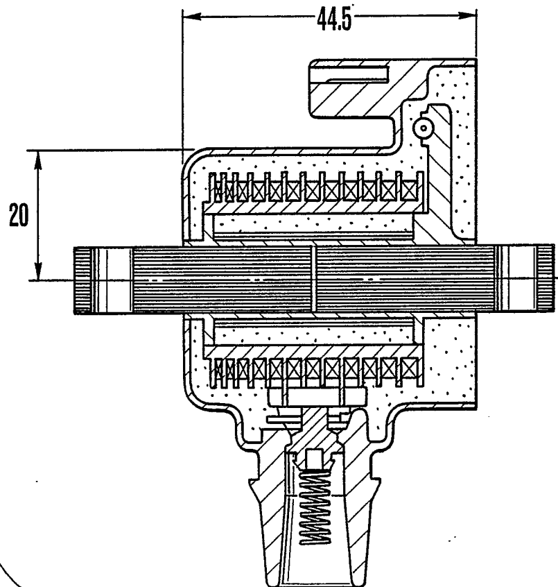
FIG.8 CONVENTIONAL IGNITION COIL
