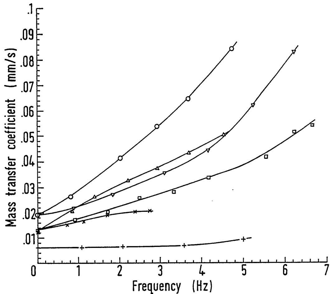
FIG. 9 Pulsatile flow.
