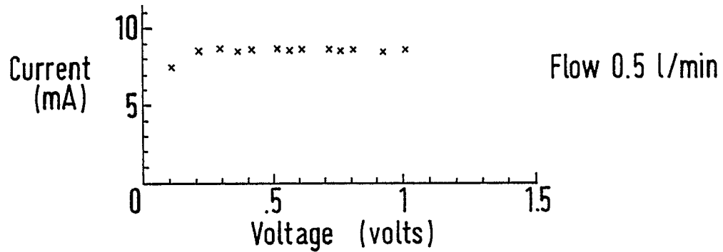
FIG. 3 Steady flow in unbaffled conduit.
