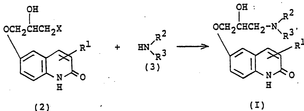
[Reaction Scheme-1]
