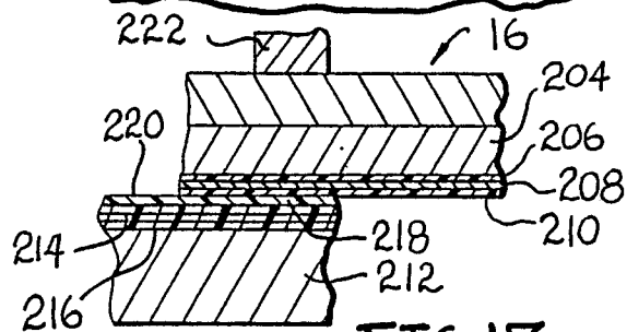
FIG. 17 (PRIOR ART).
