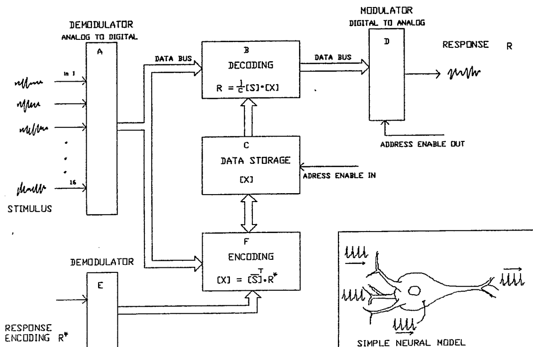
FIGURE 3 A POSSIBLE HARDWARE CONFIGURATION FOR A SINGLE NEURAL ELEMENT
