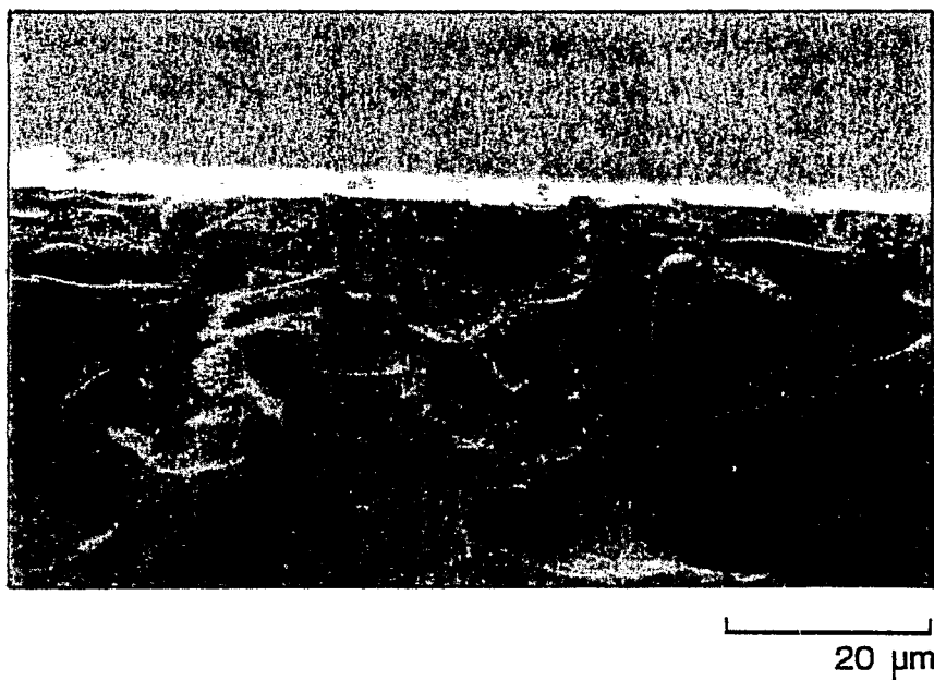
Figure 24. Example 29. SEM of a Cross Section of an Asymmetric-Membrane Capsule Wall Made of a Blend of Ethylcellulose and Cellulose Acetate. 2.5 cm = 20 μm.
