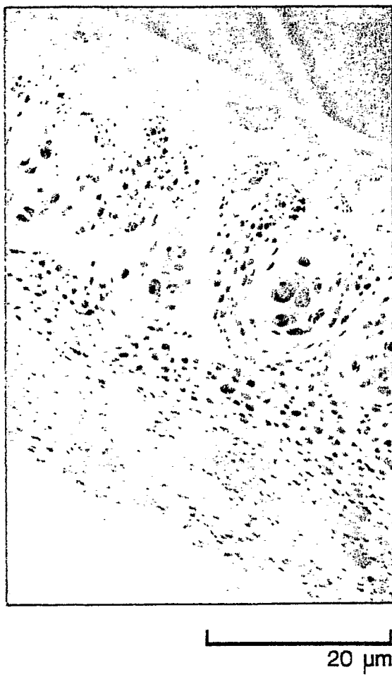
Figure 36. Example 41. SEM of a Cross Section of an Asymmetric-Membrane Capsule Wall Made of Polymethyl Methacrylate. 3.5 cm = 20 μm.
