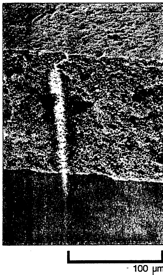
Figure 35. Example 40. SEM of a Cross Section of an Asymmetric-Membrane Capsule Wall Made of Polysulfone. 4.5 cm = 100 μm.
