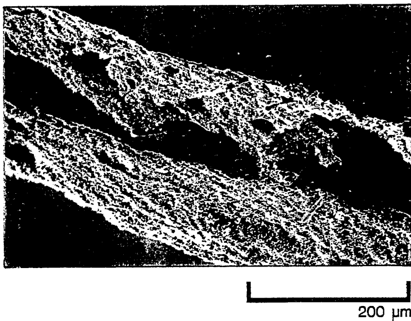
Figure 32. Example 37. SEM of a Cross Section of an Assymetric-Membrane Capsule Wall Made of Ethylenevinyl Alcohol. 4.5 cm = 200 μm.
