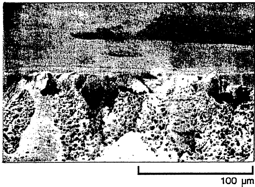
Figure 22. Example 27. SEM of a Cross Section of an Asymmetric-Membrane Capsule Wall Made of Ethylcellulose. 5 cm = 100 μm.
