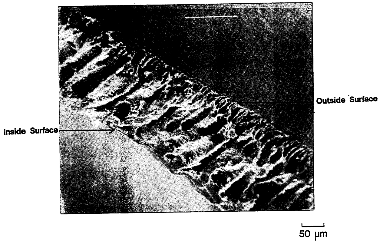
Figure 13. Example 15. SEM of a Cross Section of an Asymmetric-Membrane Capsule Wall. 1 cm = 50 \mu\text{m} .
