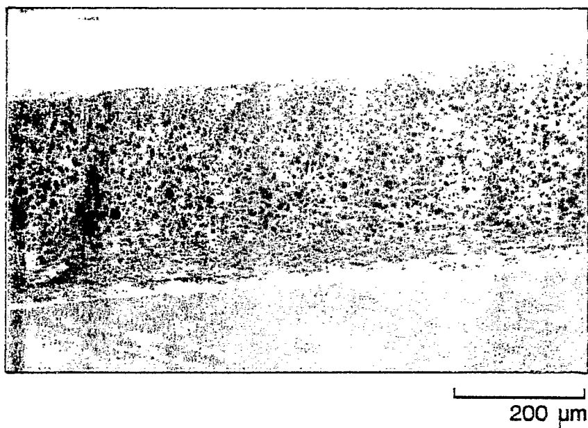
Figure 23. Example 28. SEM of a Cross Section of an Asymmetric-Membrane Capsule Wall Made of Cellulose Acetate Butyrate. 2.5 cm = 200 μm.
