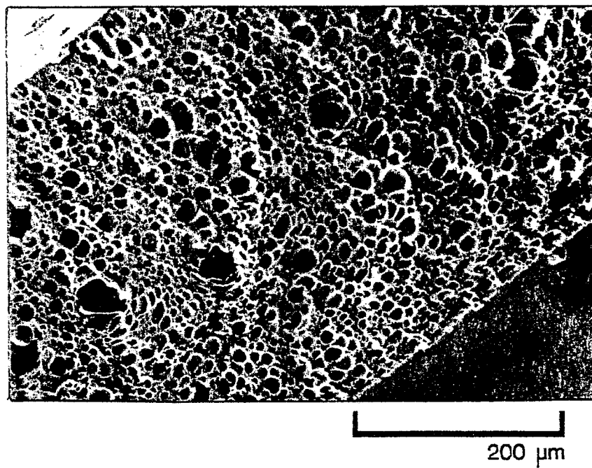
Figure 28. Example 33. SEM of a Cross Section of an Asymmetric-Membrane Capsule Wall Made of Nitrocellulose. 4 cm = 200 μm.
