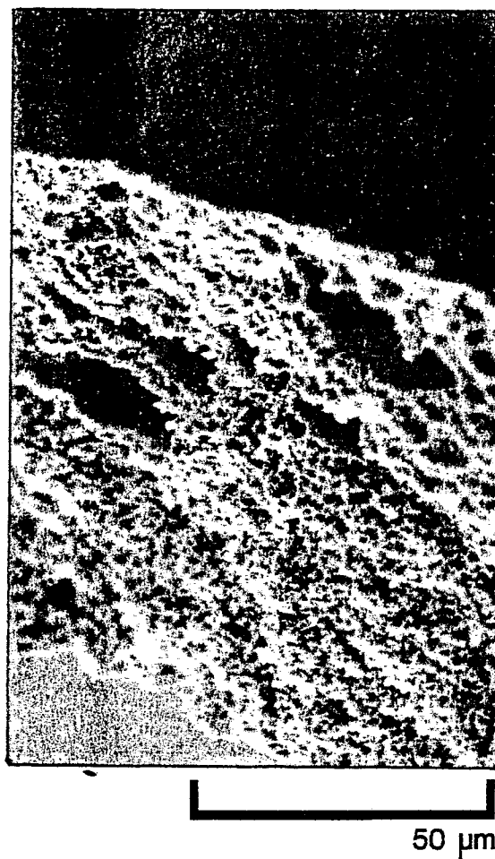
Figure 34. Example 39. SEM of a Cross Section of an Asymmetric-Membrane Capsule Wall Made of Polyvinylidene Fluoride. 4.5 cm = 50 μm.
