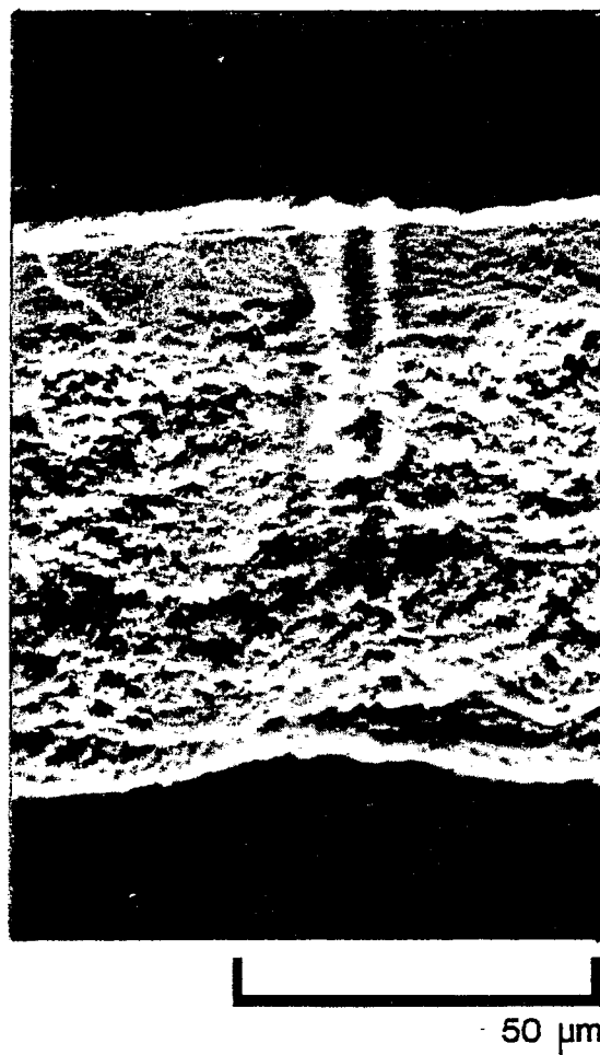
Figure 37. Example 42. SEM of a Cross Section of an Asymmetric-Membrane Capsule Wall Made of Polyamide. 4.5 cm = 50 μm.
