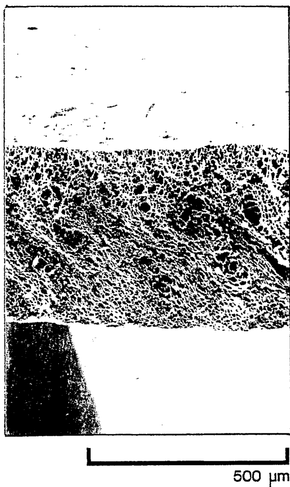
Figure 27. Example 32. SEM of a Cross Section of an Asymmetric-Membrane Capsule Wall Made of Cellulose Acetate Propionate. 5.25 cm = 500 μm.
