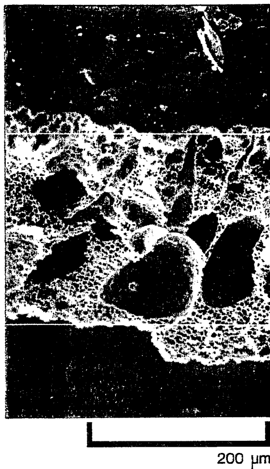
Figure 33. Example 38. SEM of a Cross Section of an Asymmetric-Membrane Capsule Wall Made of Polyurethane. 5 cm = 200 μm.
