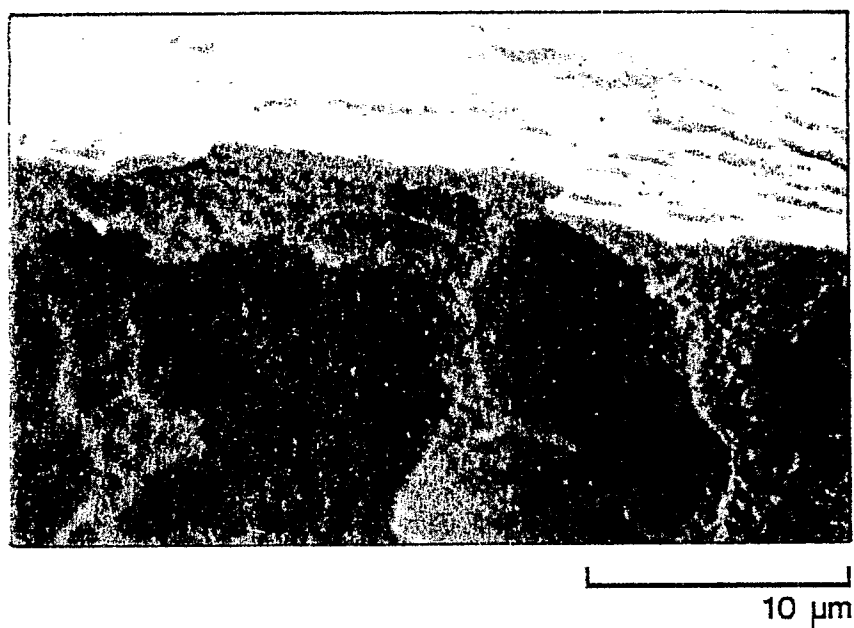
Figure 26. Example 31. SEM of a Cross Section of an Asymmetric-Membrane Capsule Wall Made of a Blend of Cellulose Acetate Butyrate and Cellulose Acetate. 3.5 cm = 10 μm.
