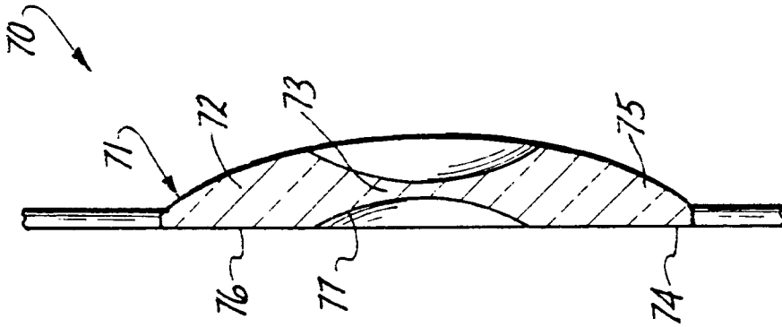
FIG 7 PRIOR ART
