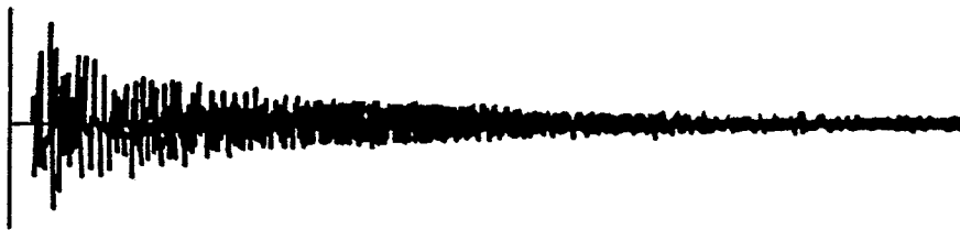
50P-100kHz SPECTRUM AND TIME RECORD
