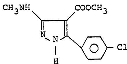
Compound C.
