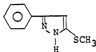
Compound C.
