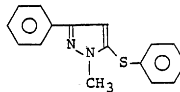
Compound D.
