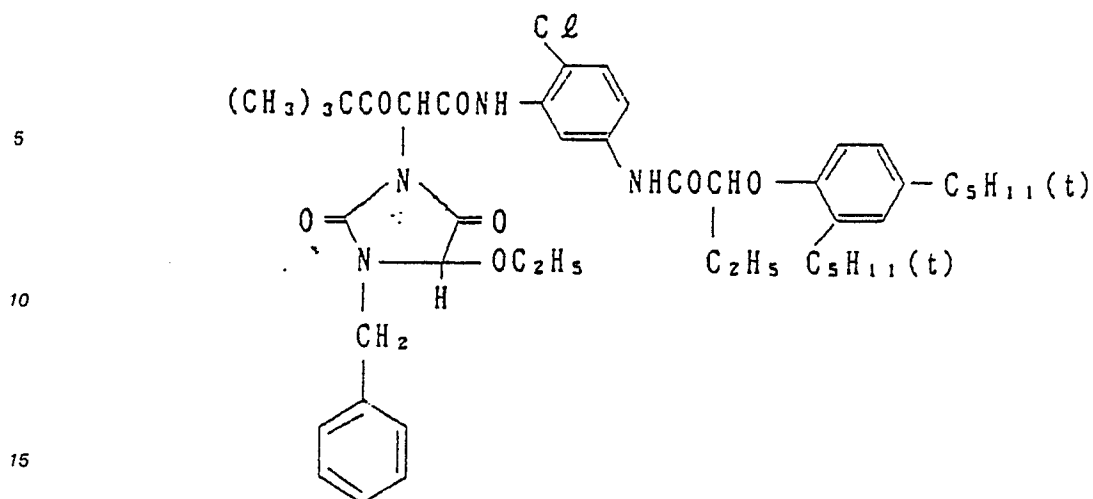
20 Color Image Stabilizer (Cpd-1)
