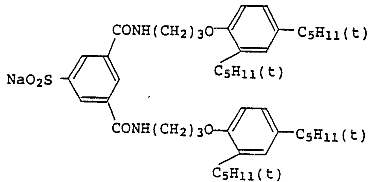
Color Image Stabilizer (Cpd-12)
