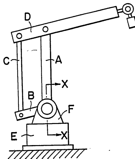
FIG. 5 PRIOR ART
