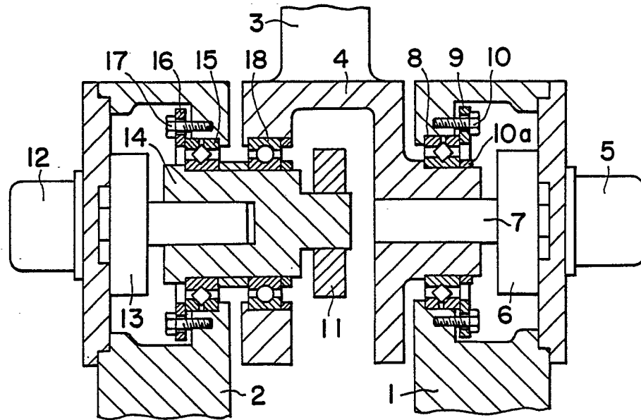
FIG. 6 PRIOR ART
