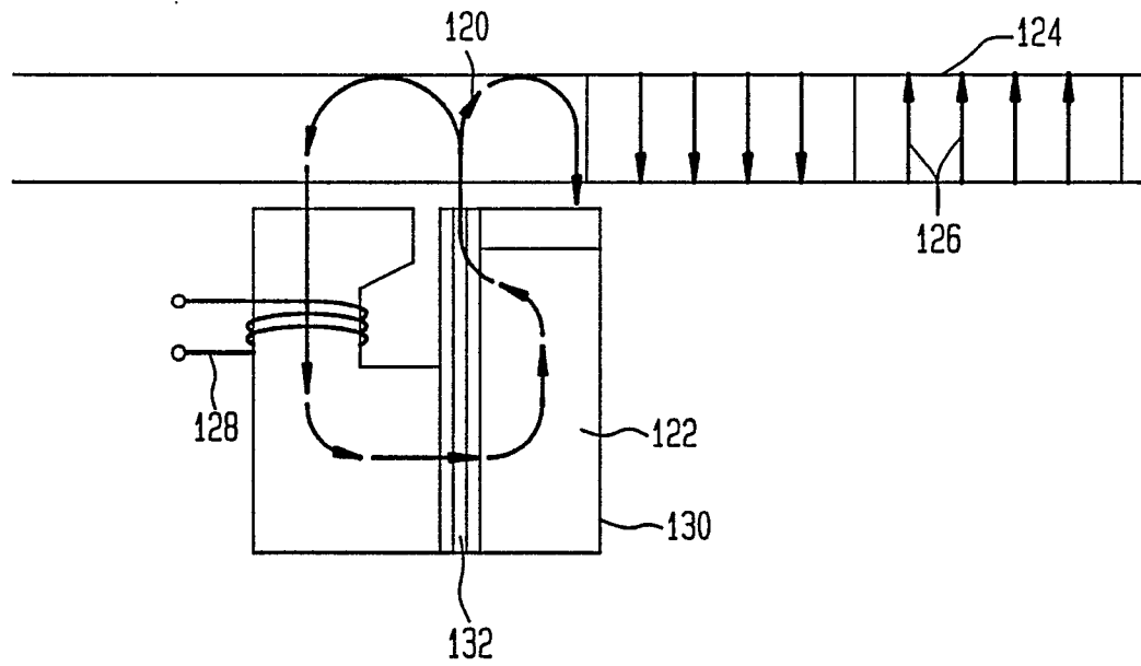
FIG. 4 (PRIOR ART)
