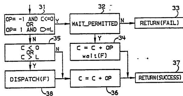
S(F, OP, WAIT_PERMITTED) FULLPHORE SIGNAL OPERATION
