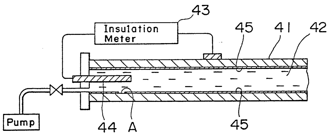
FIG.4 PRIOR ART
