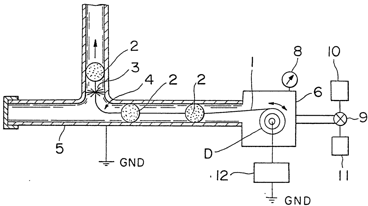
FIG.4 PRIOR ART
