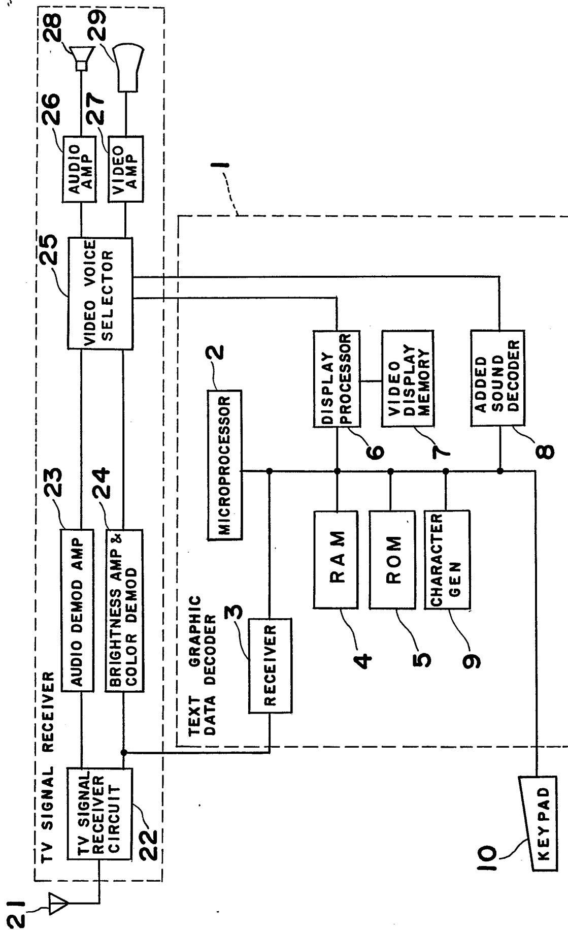
Fig. 6 PRIOR ART
