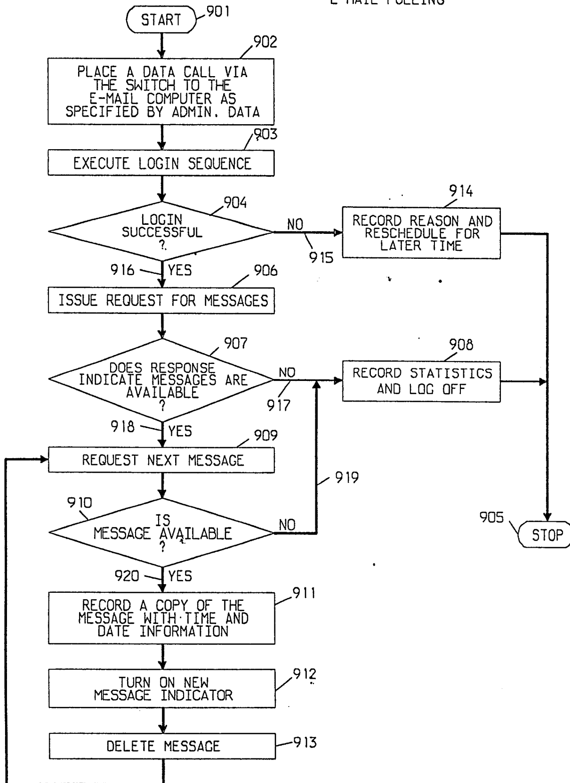
FIG. 9 E-MAIL POLLING
