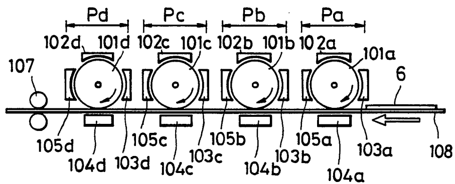
FIG. 5 PRIOR ART
