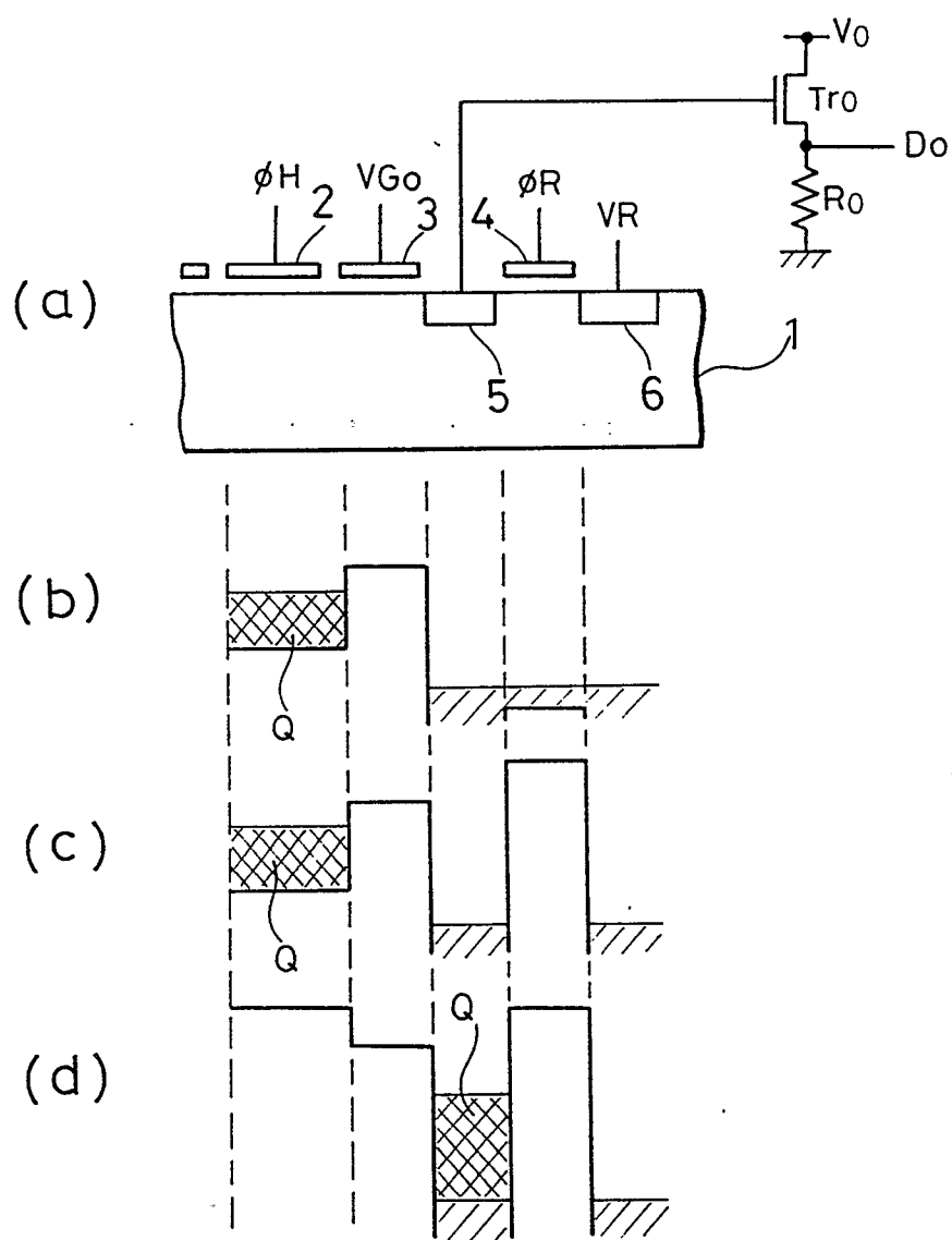
FIG. 6. (PRIOR ART)
