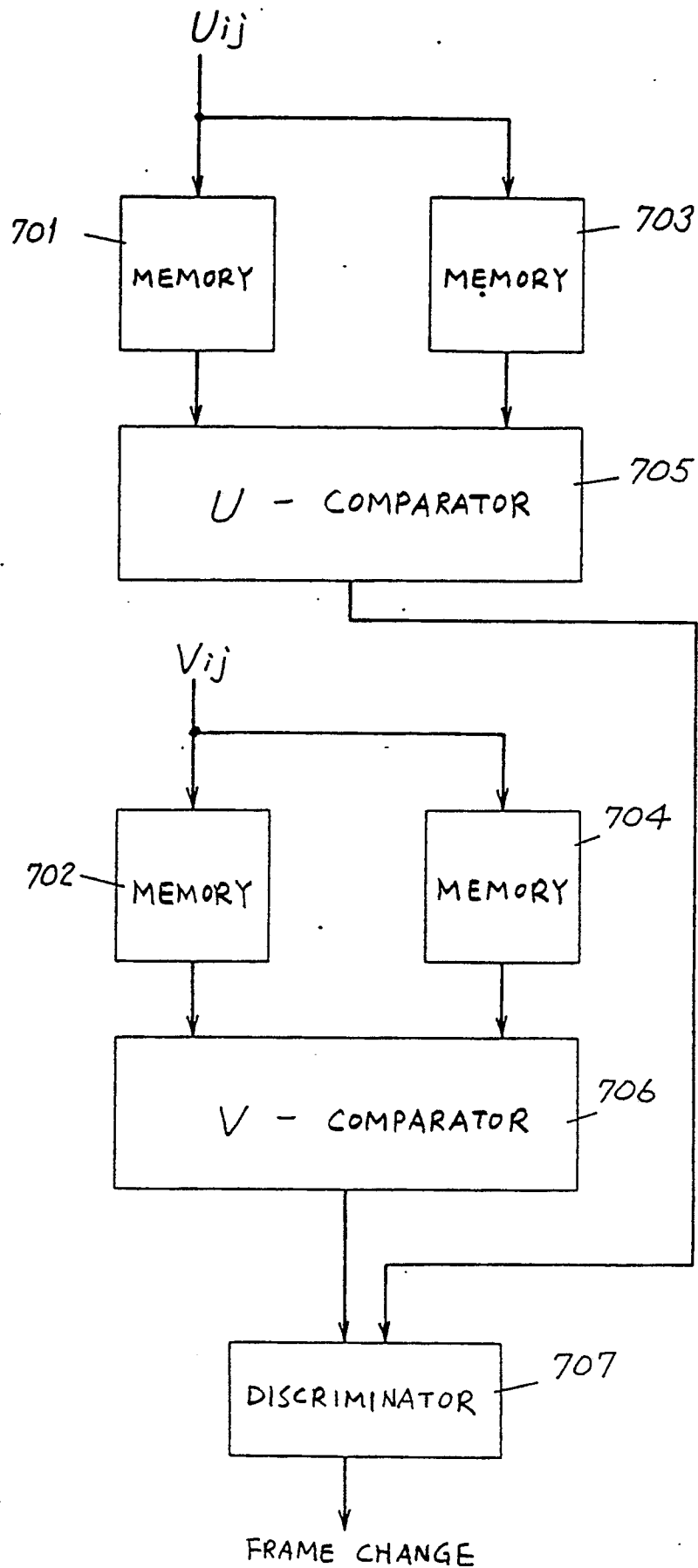
FIG. 7 (PRIOR ART)
