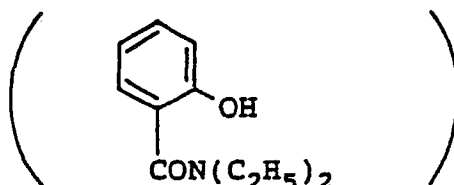
(VIII-16) O-Hydroxybenzoic Acid 2-Methylhydrazide
