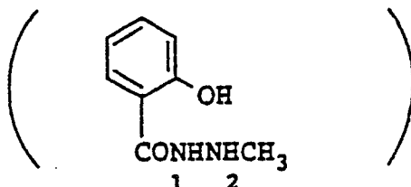
(VIII-16) O-Hydroxybenzoic Acid 2-Methylhydrazide
