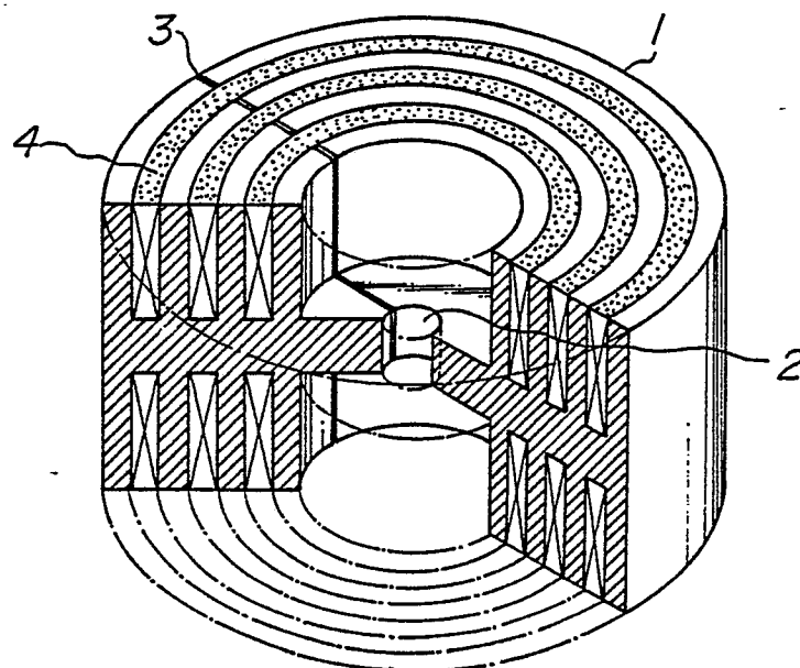
FIG. 1 PRIOR ART
