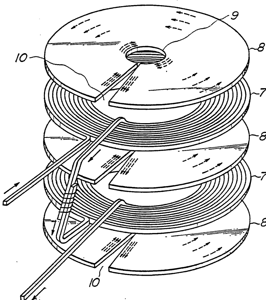
FIG. 2 PRIOR ART
