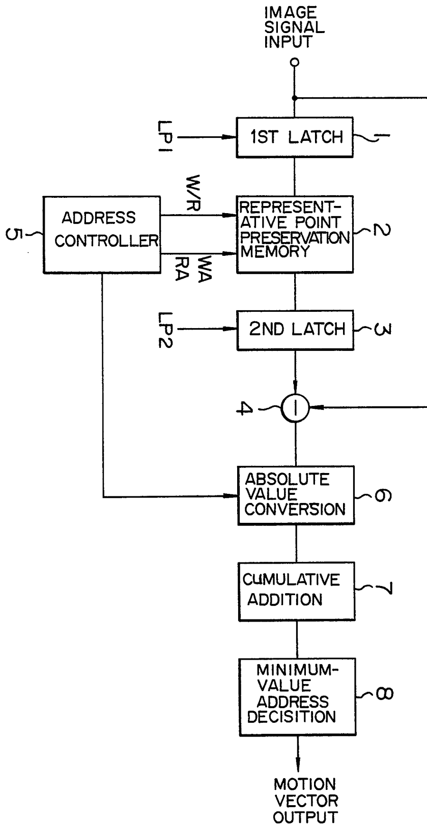
FIG. 7 PRIOR ART
