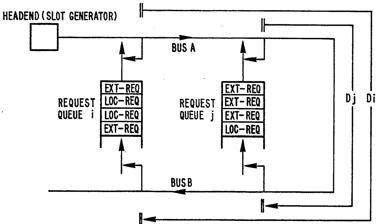
FIG. 4 PLURAL STATION FIFO QUEUES
