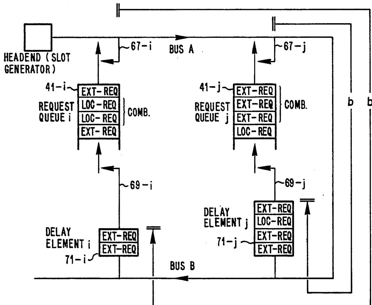
FIG. 6 PLURAL STATION FIFO QUEUES WITH DELAY
