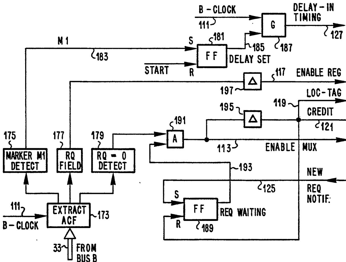
FIG. 9 BUS B CONTROLLER
