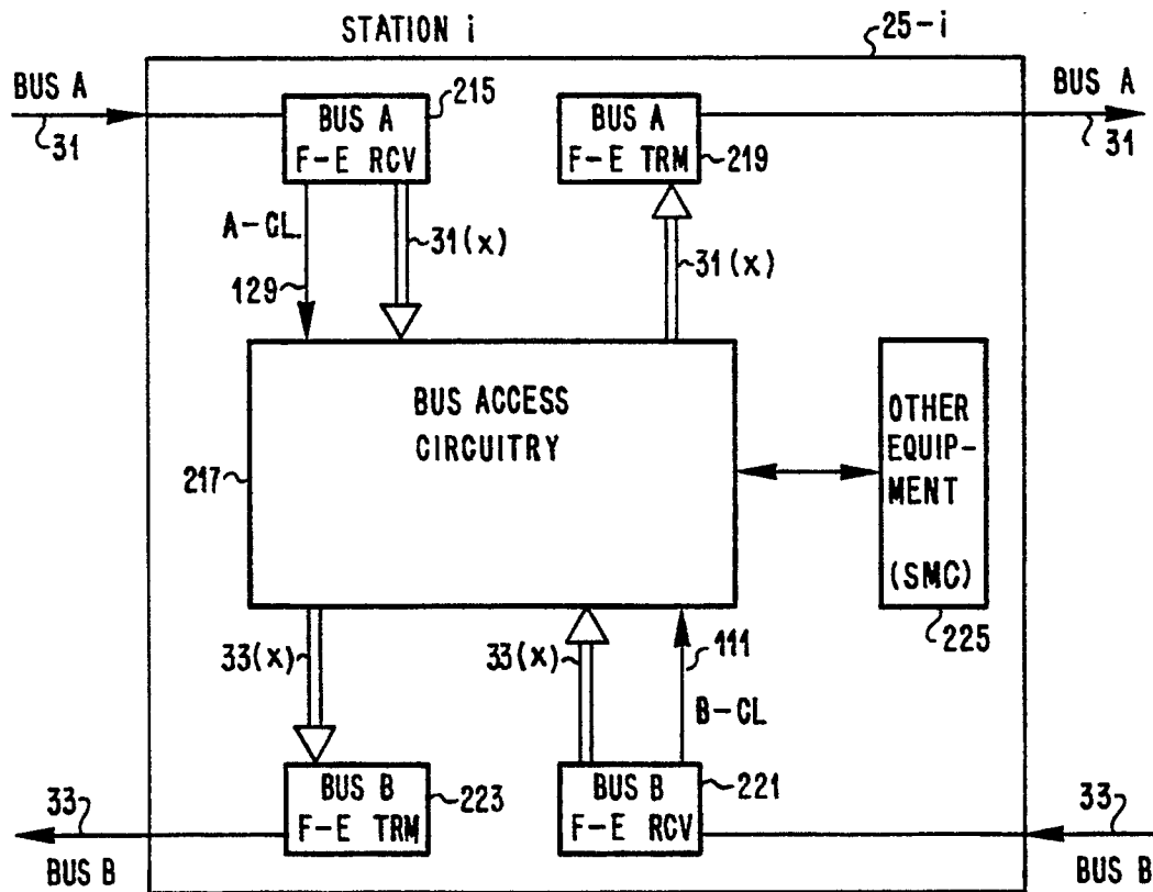
FIG. 11 SIGNAL CONVERSION BETWEEN BUS AND STATION (NODE)
