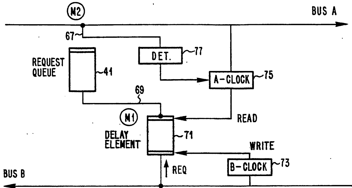
FIG. 5 REQUEST QUEUE WITH DELAY
