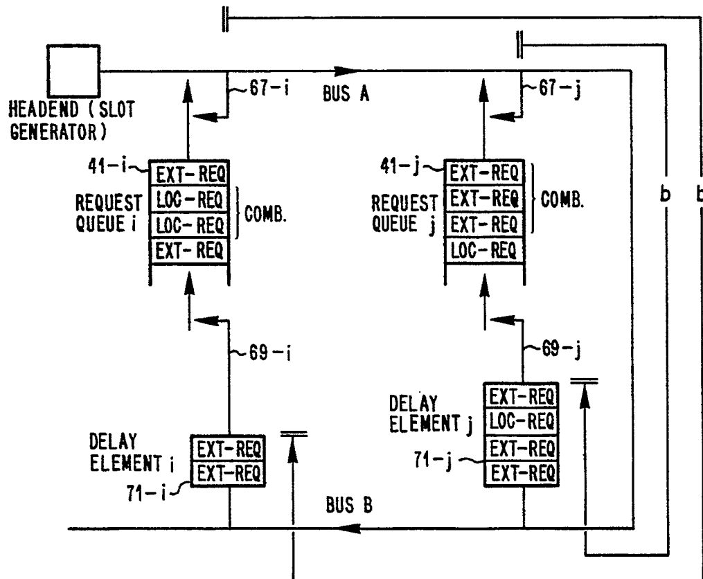
FIG. 6 PLURAL STATION FIFO QUEUES WITH DELAY
