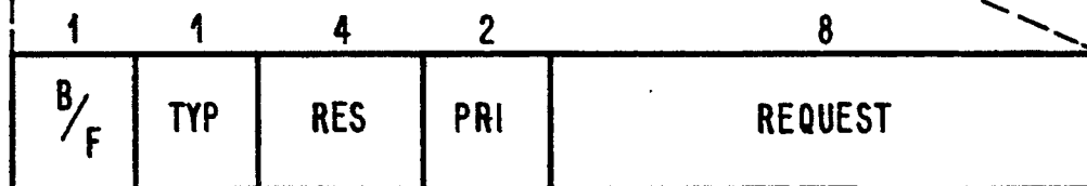
FIG. 2C ACCESS CONTROL FIELD ACF
