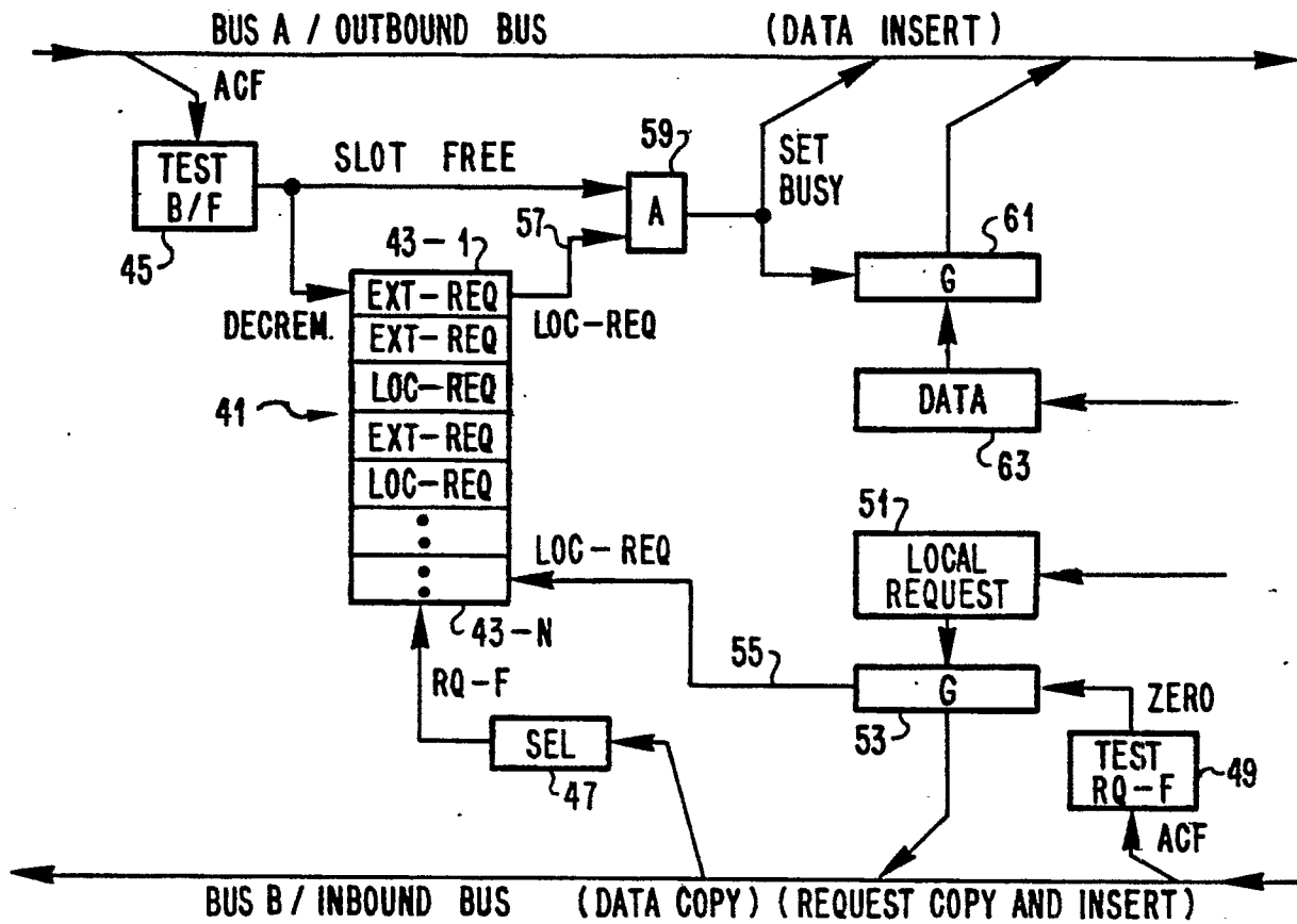
FIG. 3 BASIC FIFO REQUEST QUEUE
