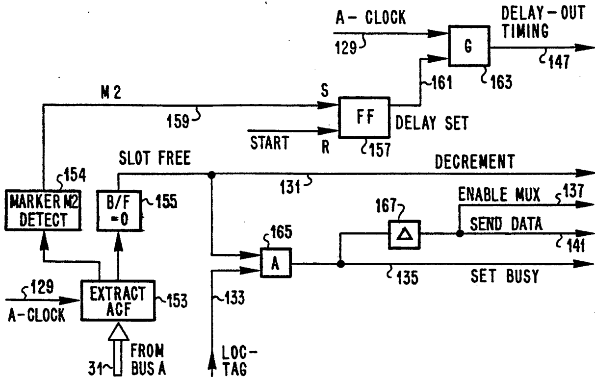
FIG. 8 BUS A CONTROLLER
